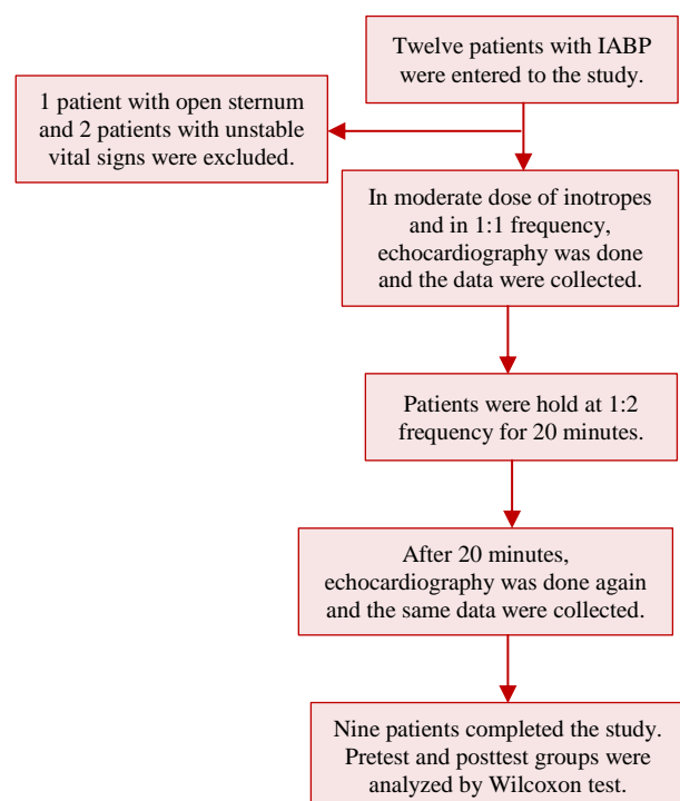
Figure 1. Study design
